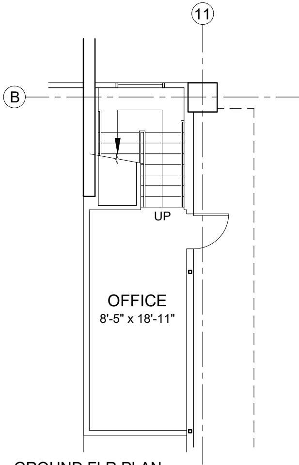
GROUND FLR PLAN
